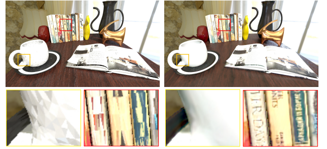
Figure 10: Ablation experiment for using higher-resolution caches calculated with equivalent preprocessing time. Left: image generated by interpolation with higher-resolution caches.
